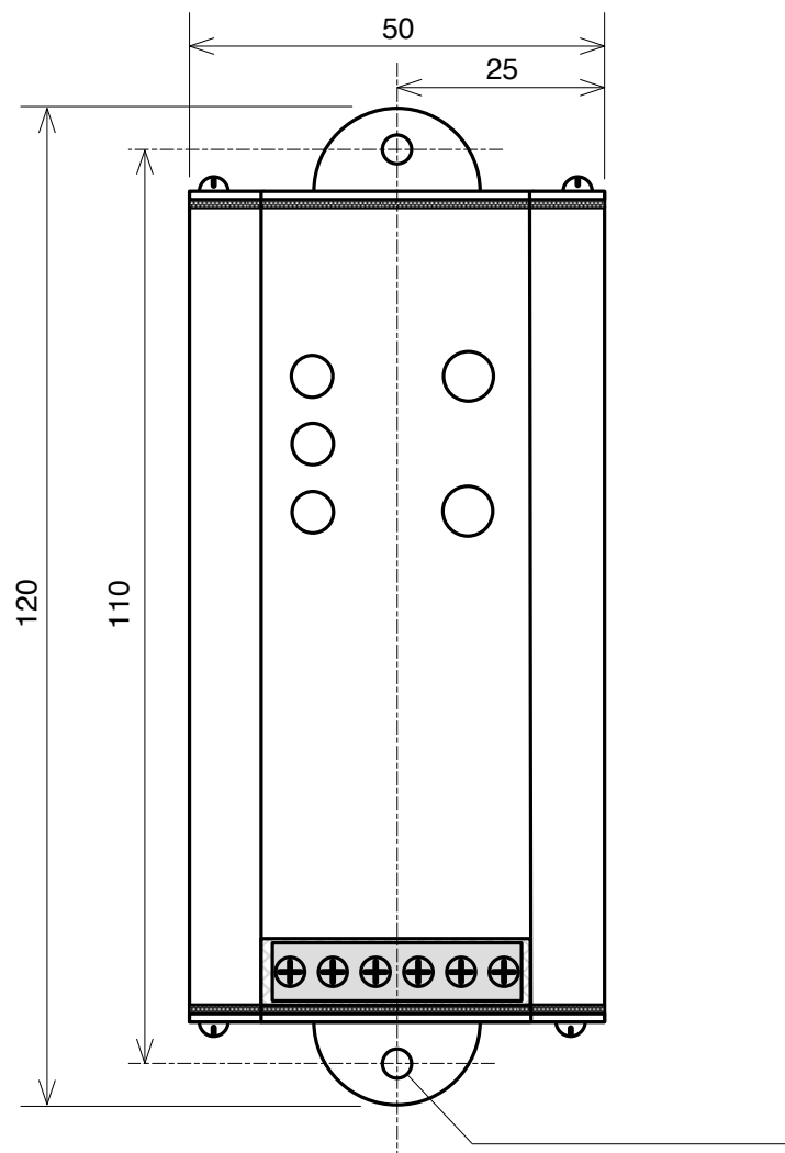
Top view (正面図)
