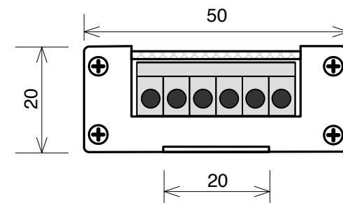
Bottom view (底面図)
